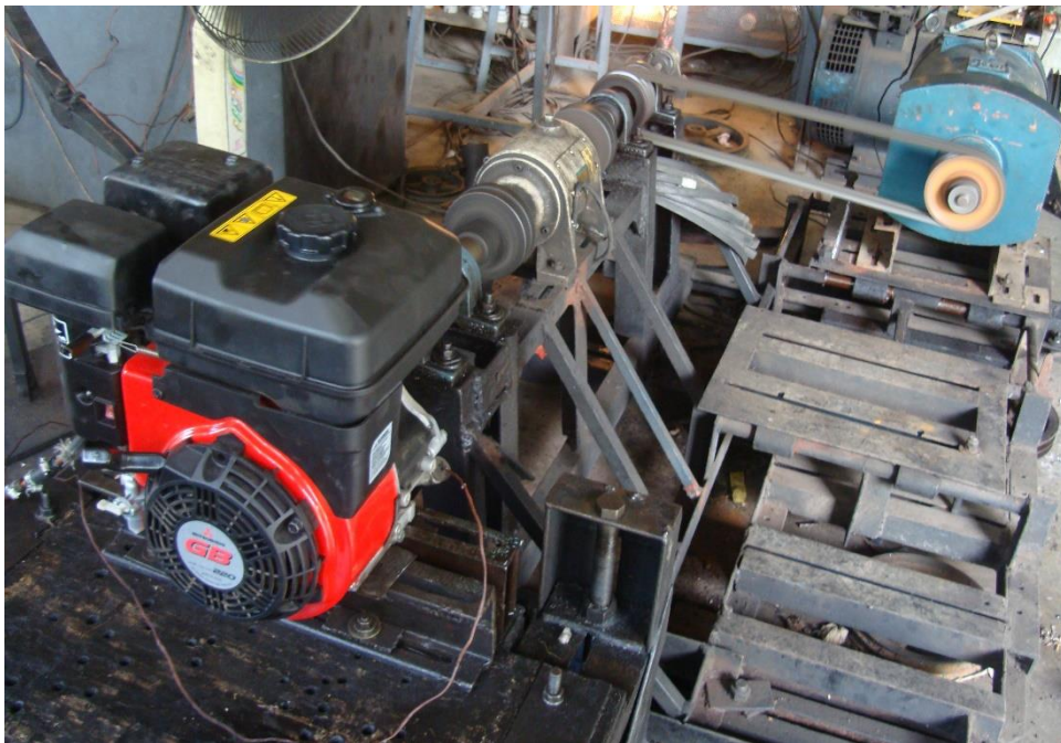
Figure 2. Test set-up of the MITSUBISHI GB200LN RTM Gasoline Engine
