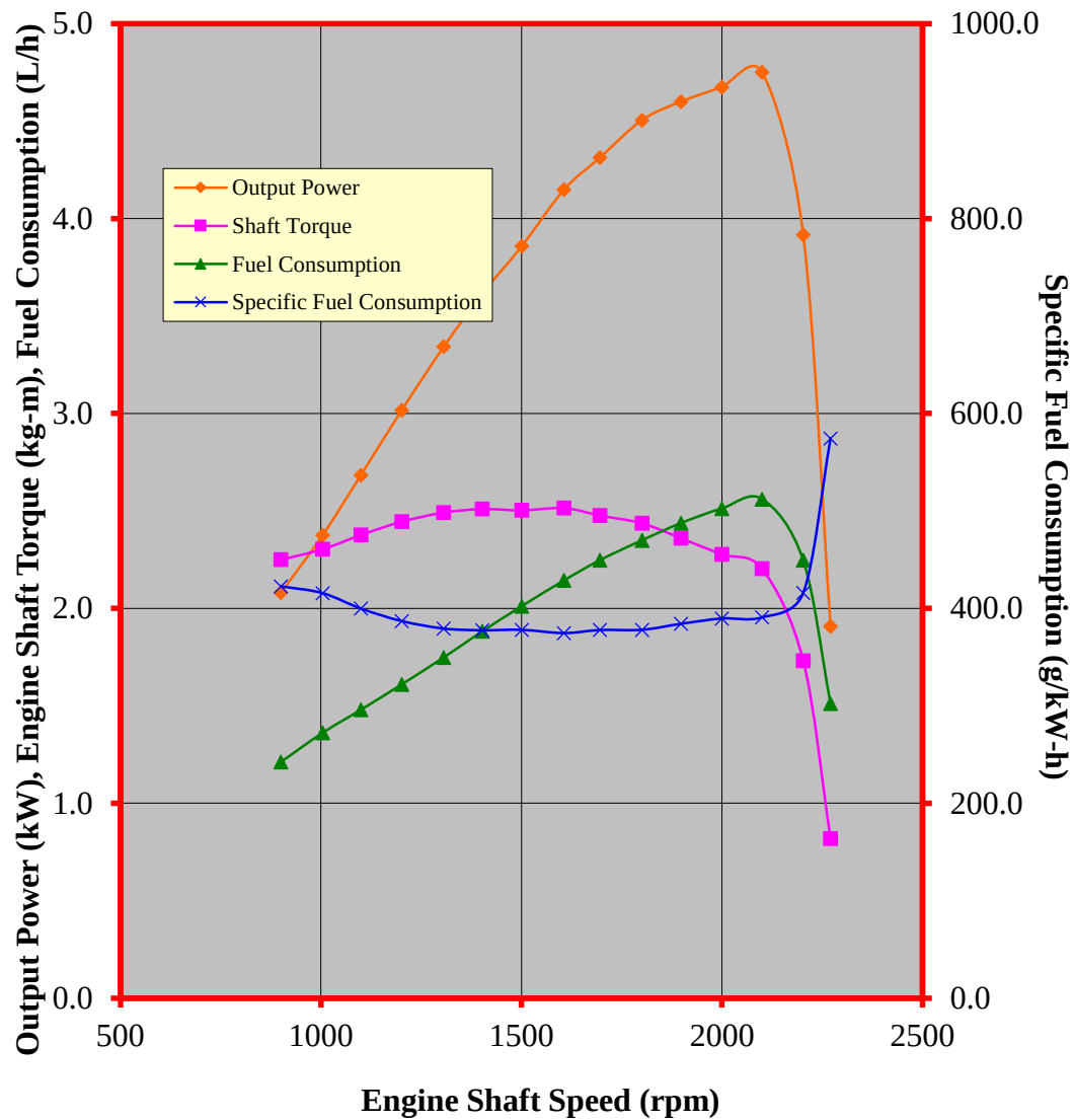
Figure 3. Performance characteristic curves of the MITSUBISHI GB-200LN RTM gasoline engine
