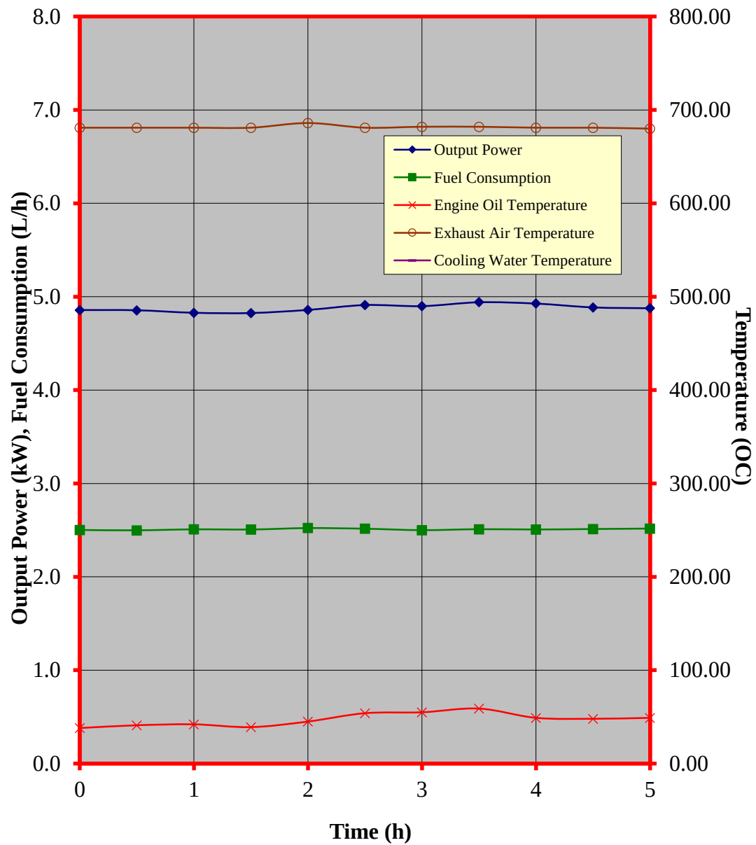
Figure 4. Performance characteristic curves during the continuous running test of the MITSUBISHI GB-200LN RTM gasoline engine
